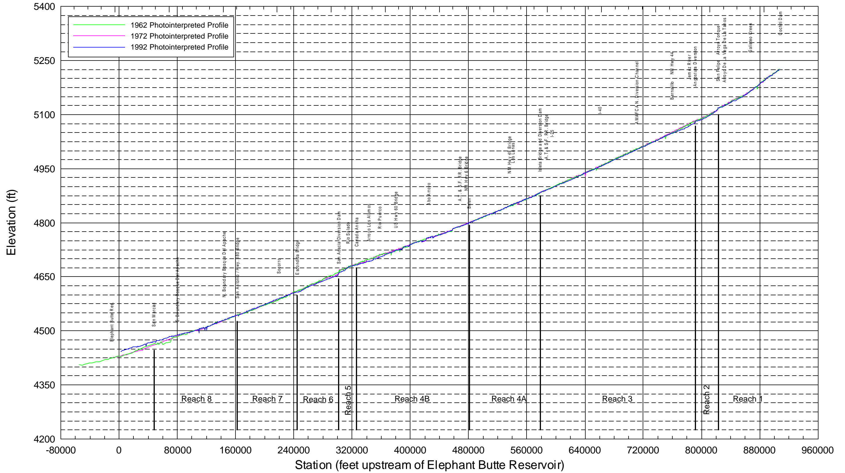
Figure 4.8. Comparative longitudinal profiles of the Middle Rio Grande based on photo-interpreted bed elevations from 1962, 1972, and 1992.
